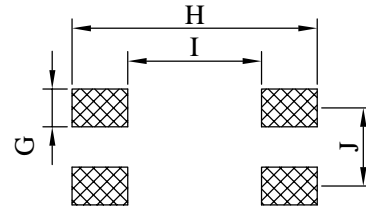
( PCB Pattern )
