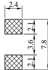
( PCB Pattern )
