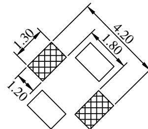
( PCB Pattern )
