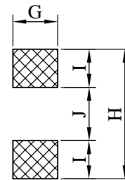
( PCB Pattern )
